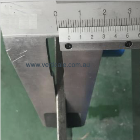
Chain Plate (Outer) 30mm (Height) x 5mm (Thickness)
